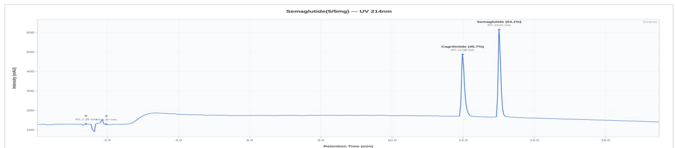
Cagrilintide/Semaglutide 5/5mg - HR-2026-5923: UV Chromatogram
