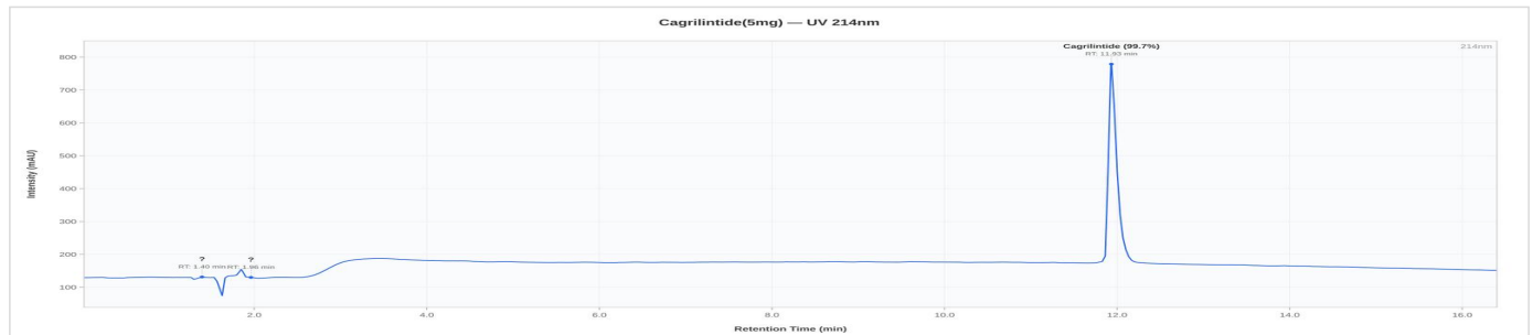
Cagrilintide 5mg - HR-2026-2608: UV Chromatogram
