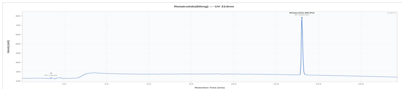
Retatrutide 60mg - HR-2026-2836: UV Chromatogram
