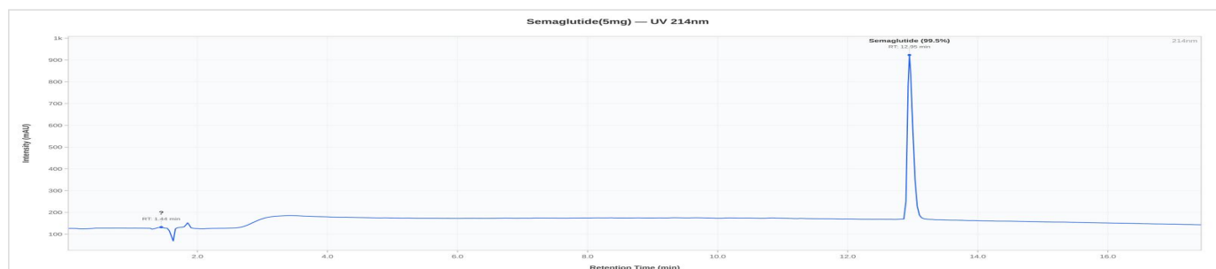
Semaglutide 5mg - HR-2026-7341: UV Chromatogram
