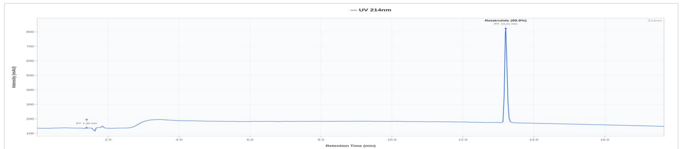
Retatrutide 20mg - HR-2026-2836: UV Chromatogram
