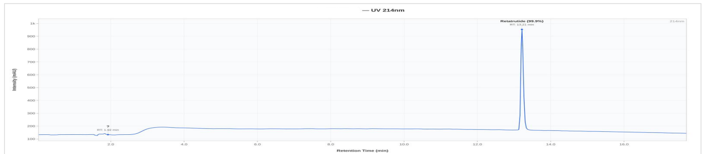
Retatrutide 40mg - HR-2026-2836: UV Chromatogram
